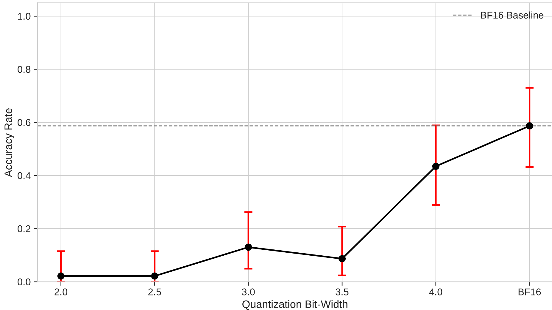
Global Zero-Shot Accuracy with 95% Confidence Intervals
