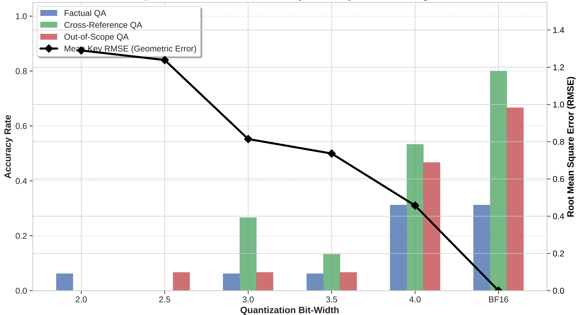
TurboQuant Phase Transition: Accuracy Recovery vs. RMSE Degradation
