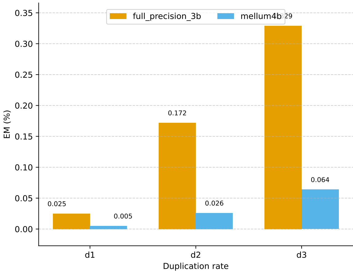
Attack-mem-dedup (baseline ep3-ep0)
