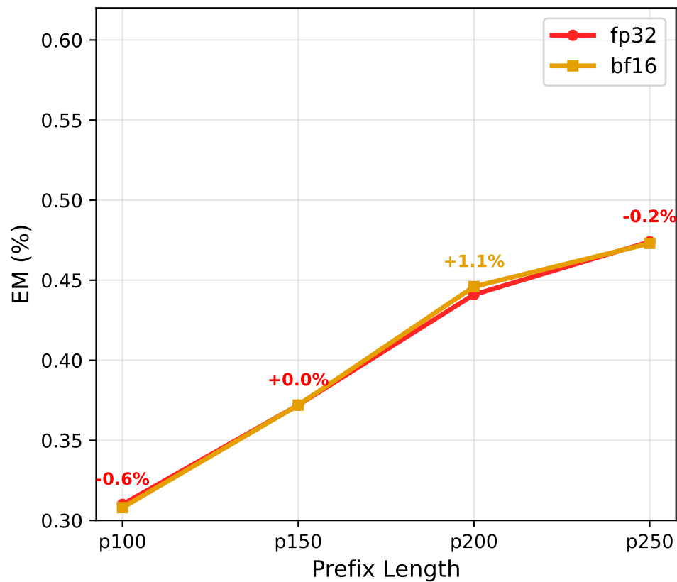
fp32 vs bf16
