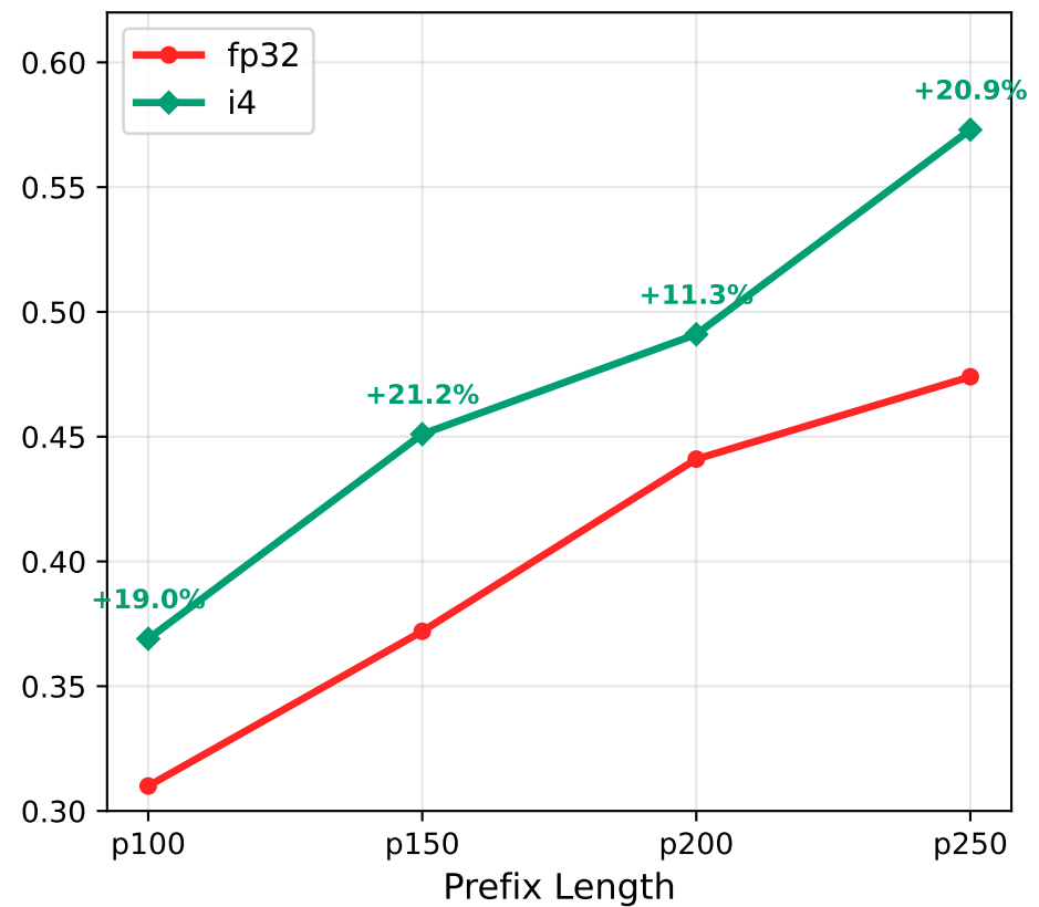
fp32 vs i4
