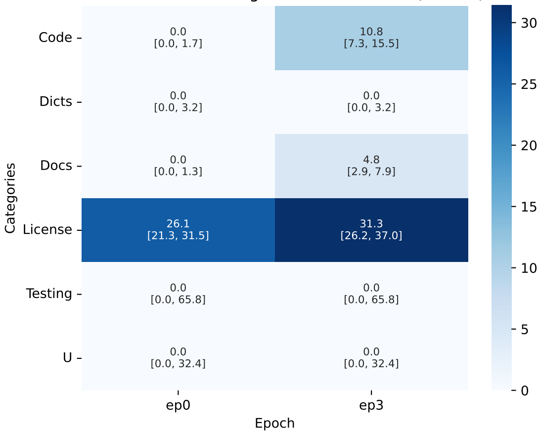
Mellum-4b Fine-tune Tags - Memorization % (95% CI)
