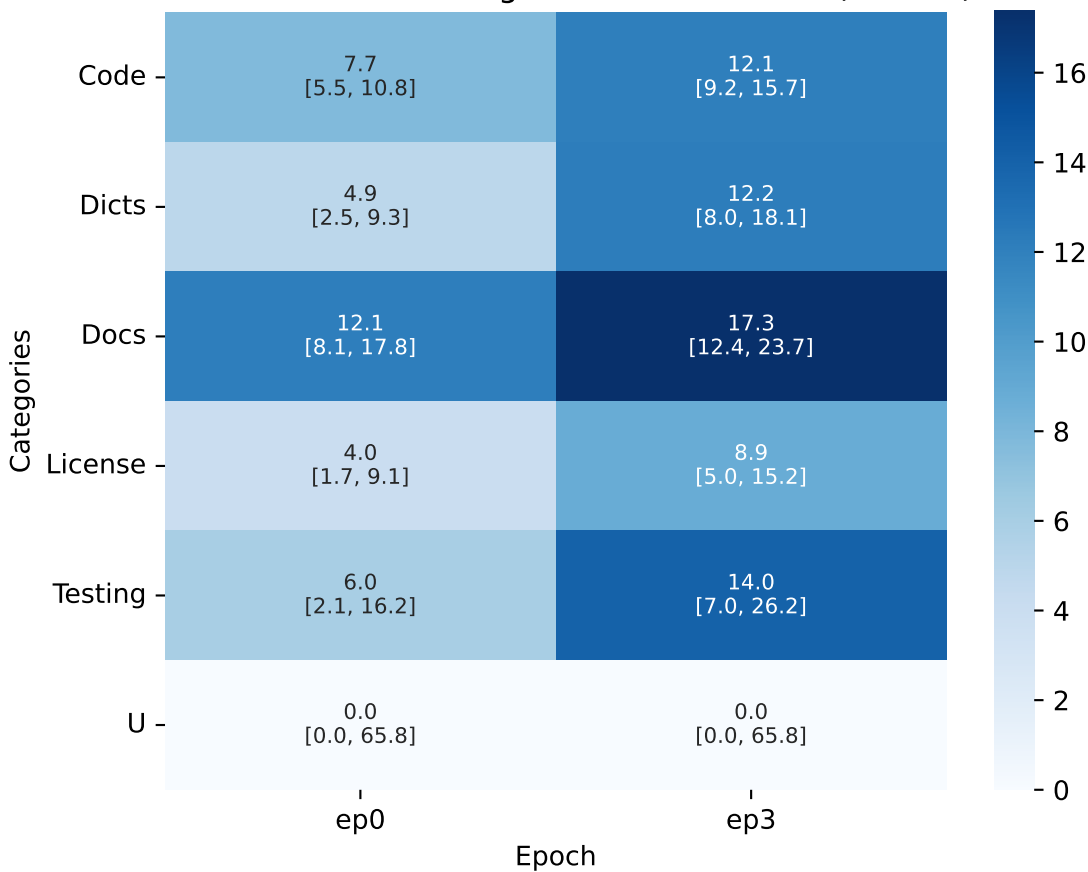
Mellum-4b Pre-train Tags - Memorization % (95% CI)
