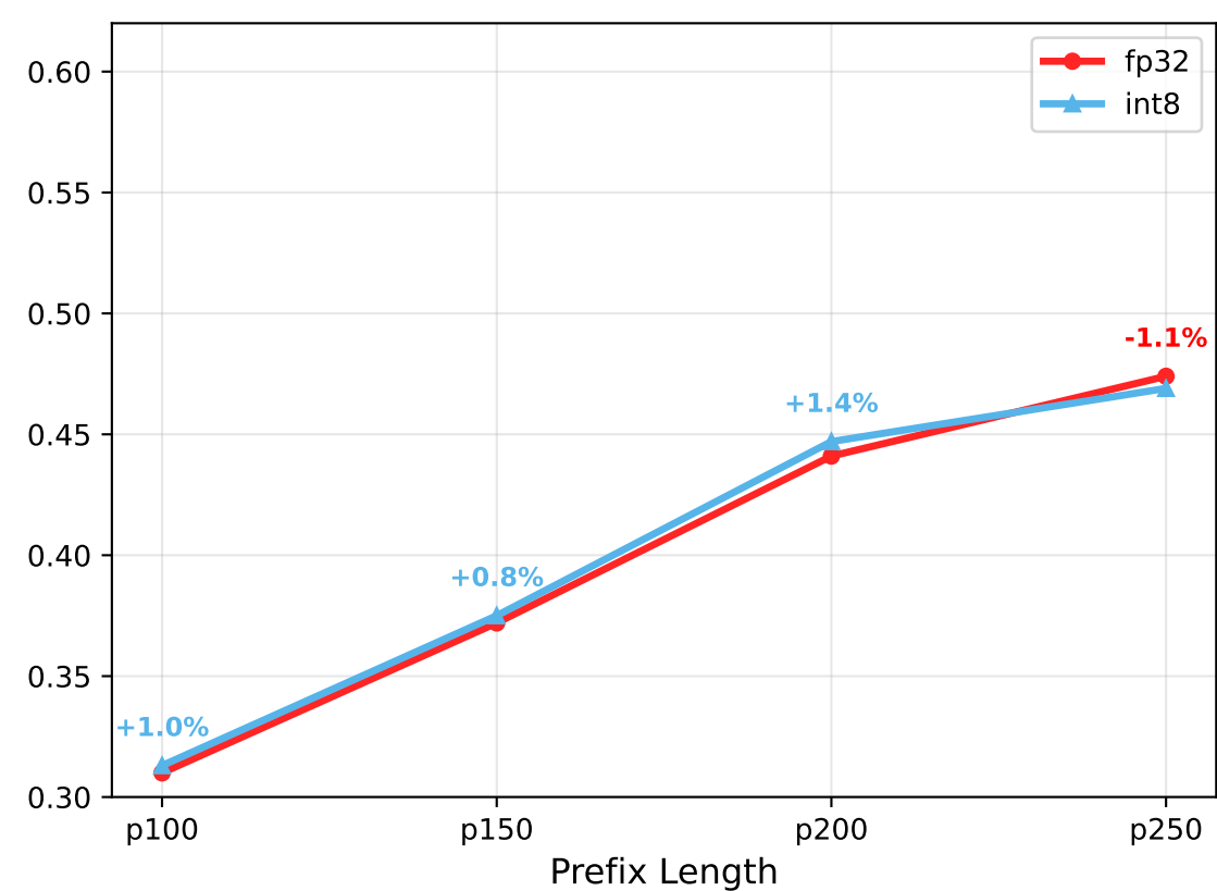
Percentages: fp32 vs int8
