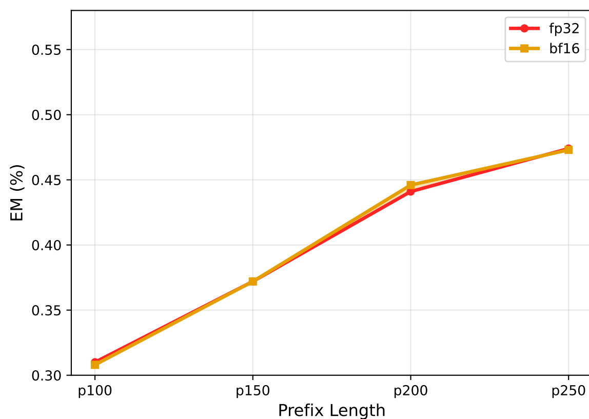
Percentages: fp32 vs bf16
