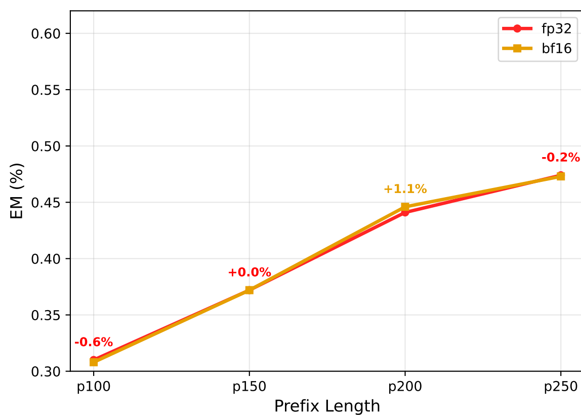
Percentages: fp32 vs bf16
