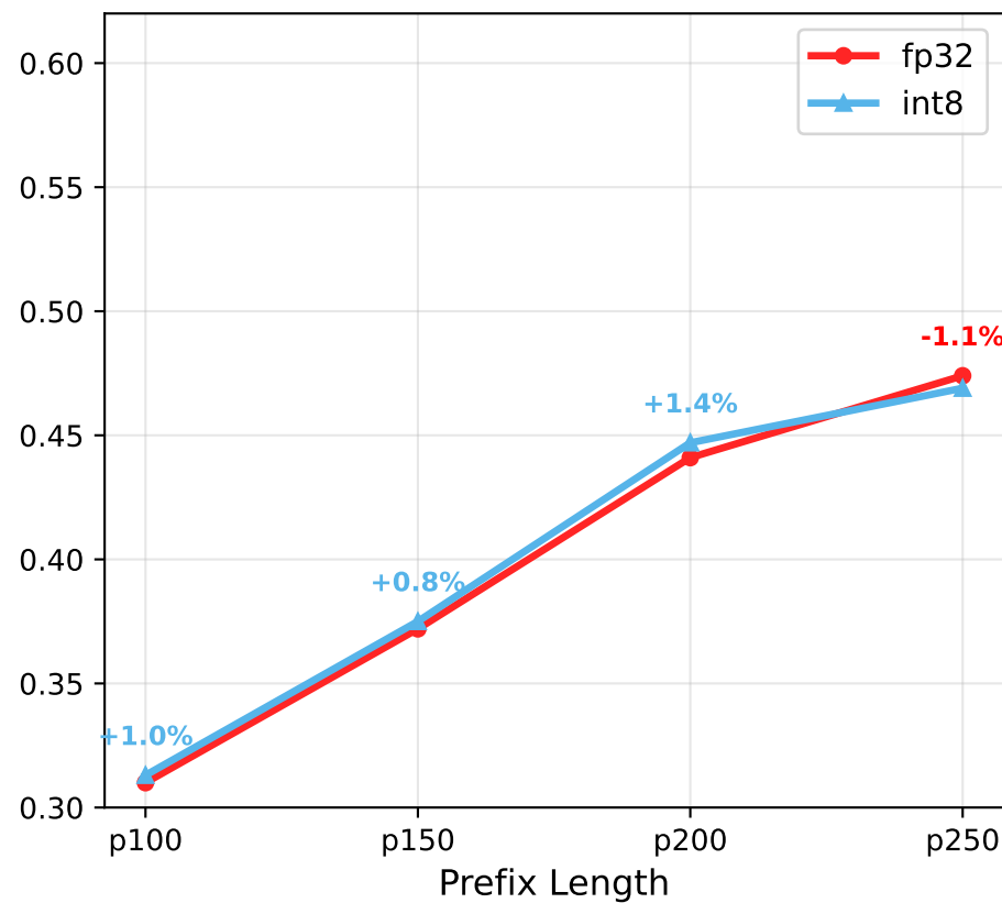
fp32 vs int8
