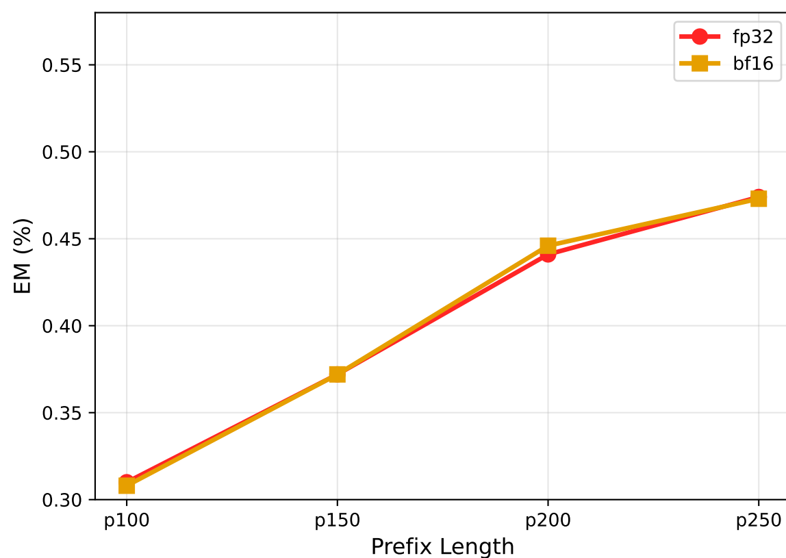
Clean: fp32 vs bf16
