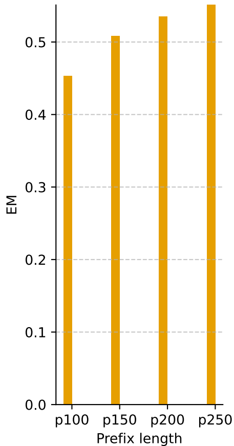
bf16
