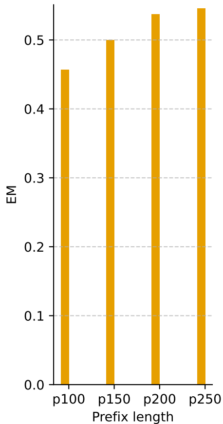
int8
