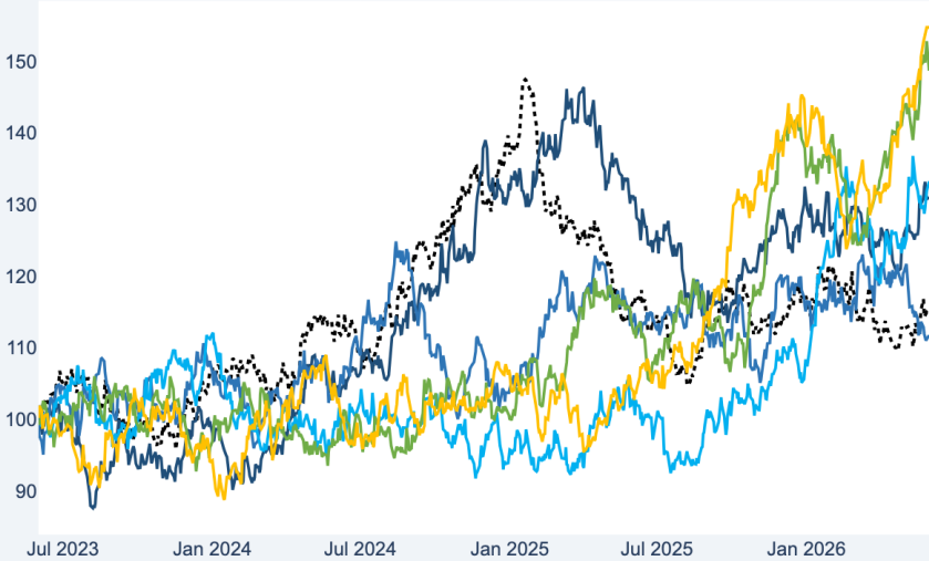
NAV vs Benchmark — Top 5 Funds (3Y, Base 100)
