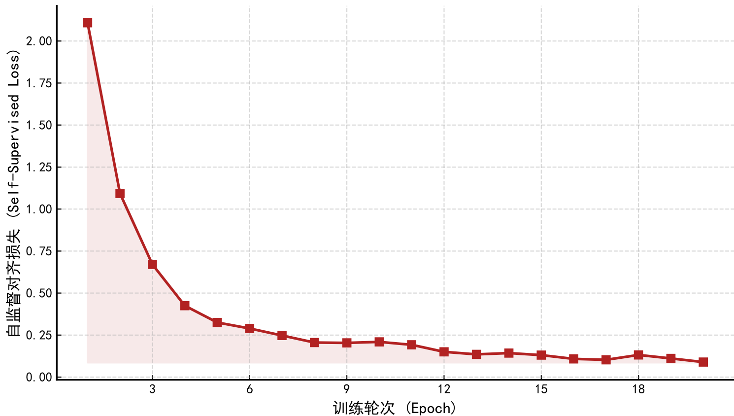
模型自监督伪标签对齐损失收敛曲线 (Alignment Loss)
