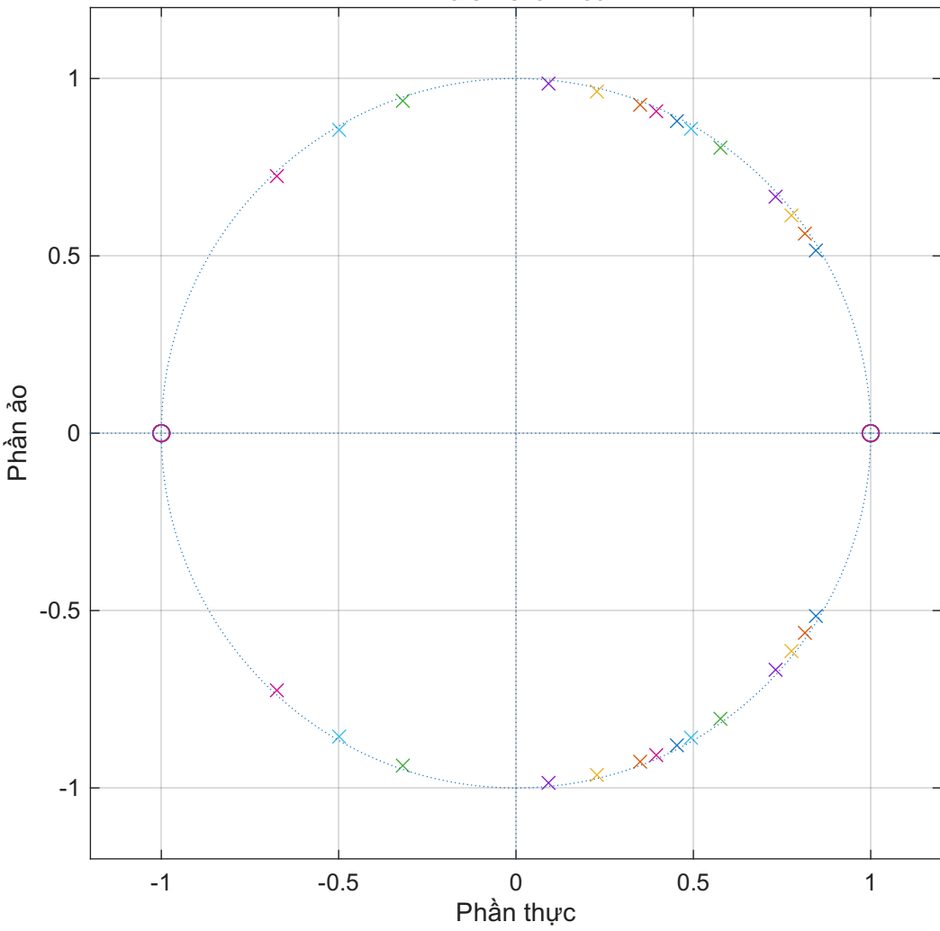
Pole-Zero Plot
