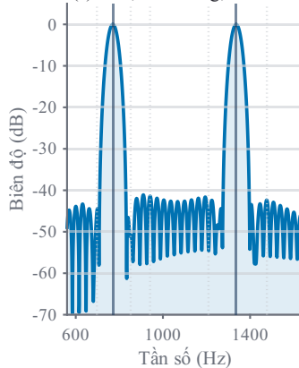
(c) FFT, Hamming, N = 256
