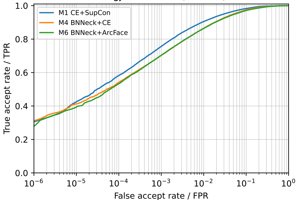
Tongji strict ROC (S2->S1)
