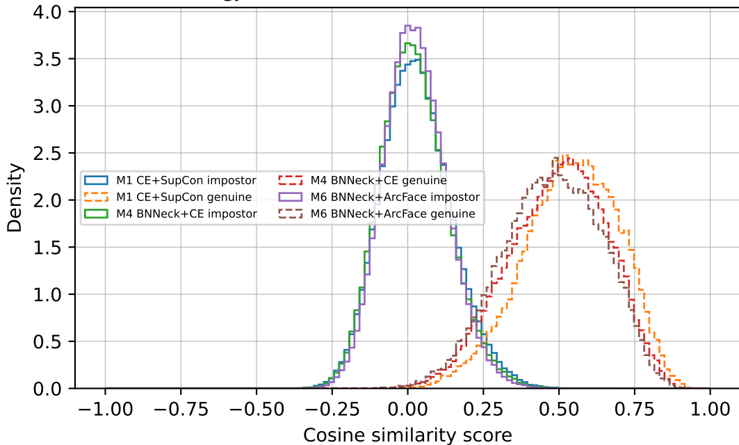
Tongji strict score distributions (S2->S1)
