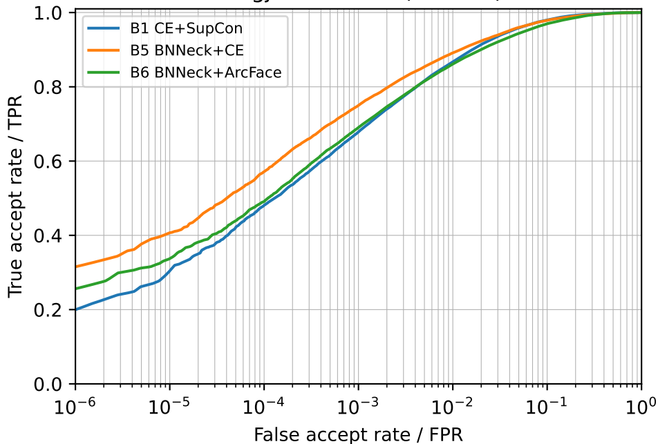
Tongji strict ROC (S1->S2)
