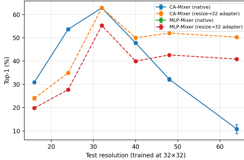
(b) Zero-shot accuracy across resolutions.
