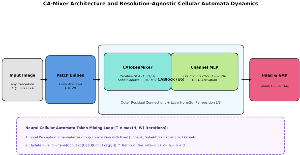
Figure 3: Macro-architecture of CA-Mixer and the Neural Cellular Automata (NCA) iterative perception and update dynamics.
