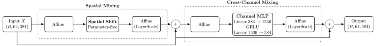
(b) Shift-ResMLP block structure separating spatial mixing from cross-channel mixing.
