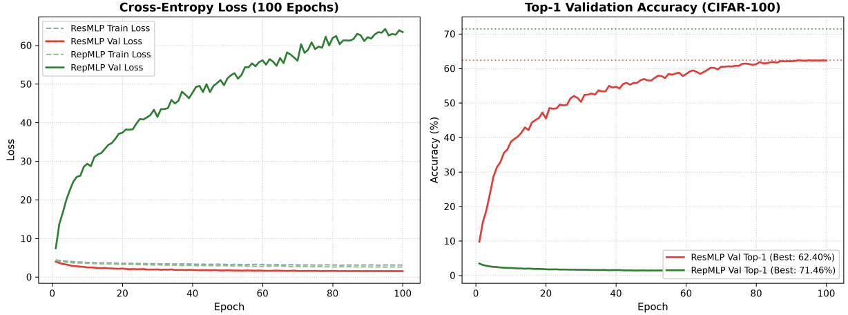
Figure 1: Training curves across 100 epochs on CIFAR-100: (Left) Cross-entropy loss on train and validation sets; (Right) Top-1 validation accuracy showing warmup, mid-phase training, and final convergence.
