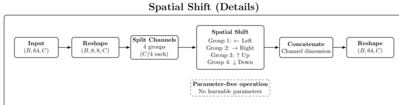
(c) Parameter-free 4-direction coordinate shift mechanism.
