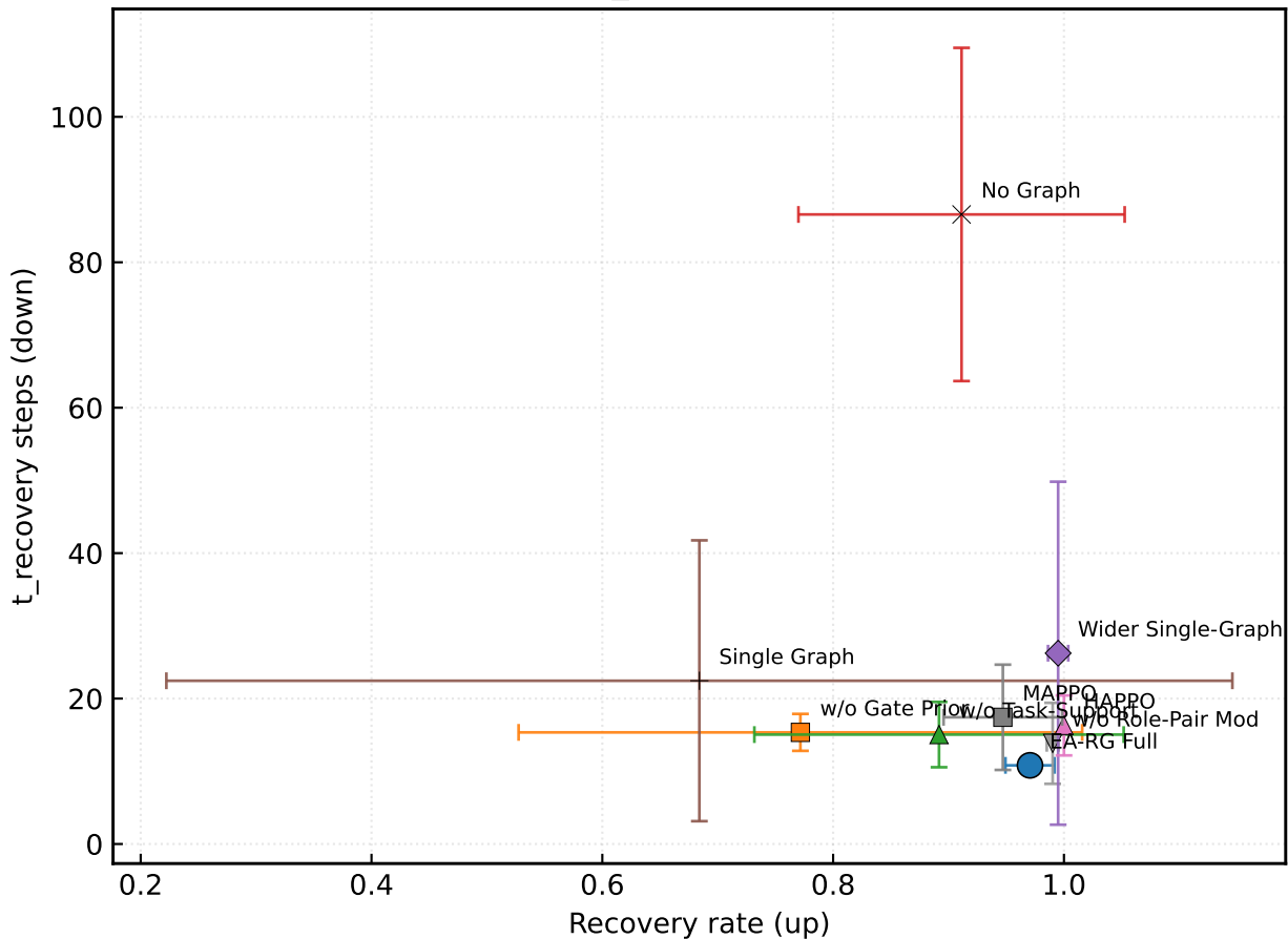
Recovery rate vs t_recovery steps (n=3 seeds)
