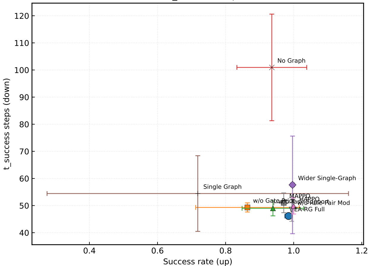
Success rate vs t_{\text{success}} steps (n=3 seeds)
