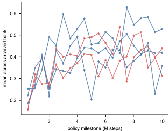
DRTP-UTR Jensen-Shannon divergence
