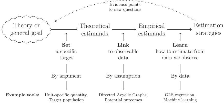
Figure 1. Three Critical Choices in Quantitative Social Science Arguments
