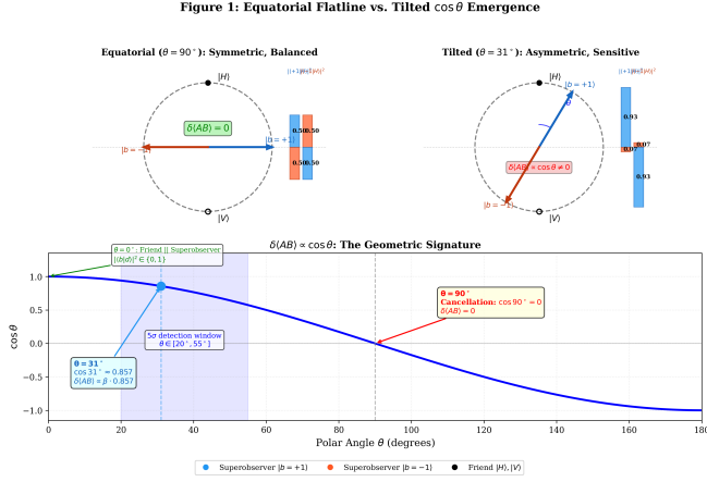
FIG. 1. Equatorial flatline vs. tilted \cos \theta emergence. Left panel: Bloch sphere showing Superobserver measurement axis at equator ( \theta = \pi/2 ). All four overlap magnitudes |\langle b|d\rangle|^2 = 1/2 — symmetric, balanced, \delta\langle AB\rangle = 0 identically (flatline). Right panel: axis tilted to \theta = 31^\circ . Overlap asymmetry emerges: |\langle +1|H\rangle|^2 = \cos^2(15.5^\circ) \approx 0.93 , |\langle -1|H\rangle|^2 = \sin^2(15.5^\circ) \approx 0.07 — the Superobserver basis aligns preferentially with one Friend outcome. Lower panel: predicted \delta\langle AB\rangle(\theta) curve (numerical), showing the exact null at \theta = 90^\circ (equator) and the onset of non-zero signal as \theta departs from the equatorial plane. The single-waveplate modification moves the measurement from the flatline at 90^\circ to the sensitive region at 31^\circ (dashed vertical line).
