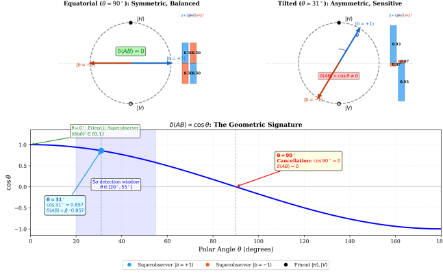
FIG. 1. Equatorial flatline vs. tilted \cos\theta emergence. Left panel: Bloch sphere showing Superobserver measurement axis at equator ( \theta = \pi/2 ). All four overlap magnitudes |\langle b|d\rangle|^2 = 1/2 — symmetric, balanced, \delta\langle AB\rangle = 0 identically (flatline). Right panel: axis tilted to \theta = 31^\circ . Overlap asymmetry emerges: |\langle +1|H\rangle|^2 = \cos^2(15.5^\circ) \approx 0.93 , |\langle -1|H\rangle|^2 = \sin^2(15.5^\circ) \approx 0.07 — the Superobserver basis aligns preferentially with one Friend outcome. Lower panel: predicted \delta\langle AB\rangle \propto \cos\theta curve, showing the exact null at \theta = 90^\circ (equator) and the linear onset as \theta departs from the equatorial plane. The single-waveplate modification moves the measurement from the flatline at 90^\circ to the sensitive region at 31^\circ (dashed vertical line).
