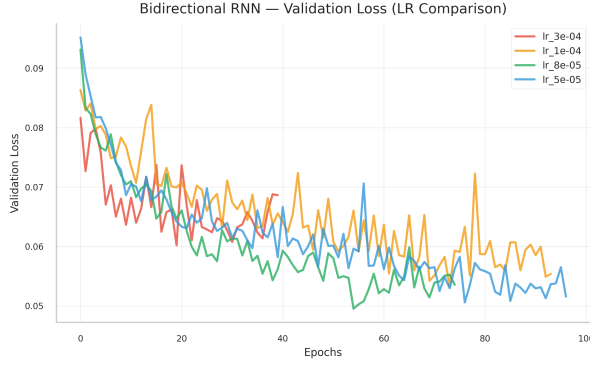
(a) Bi-RNN validation loss.
