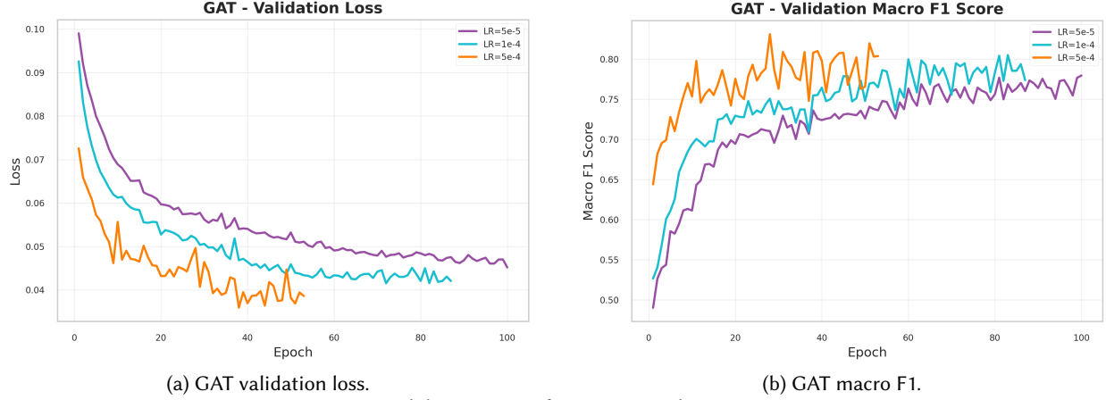
Fig. 10. Validation curves for GAT across learning rates.
