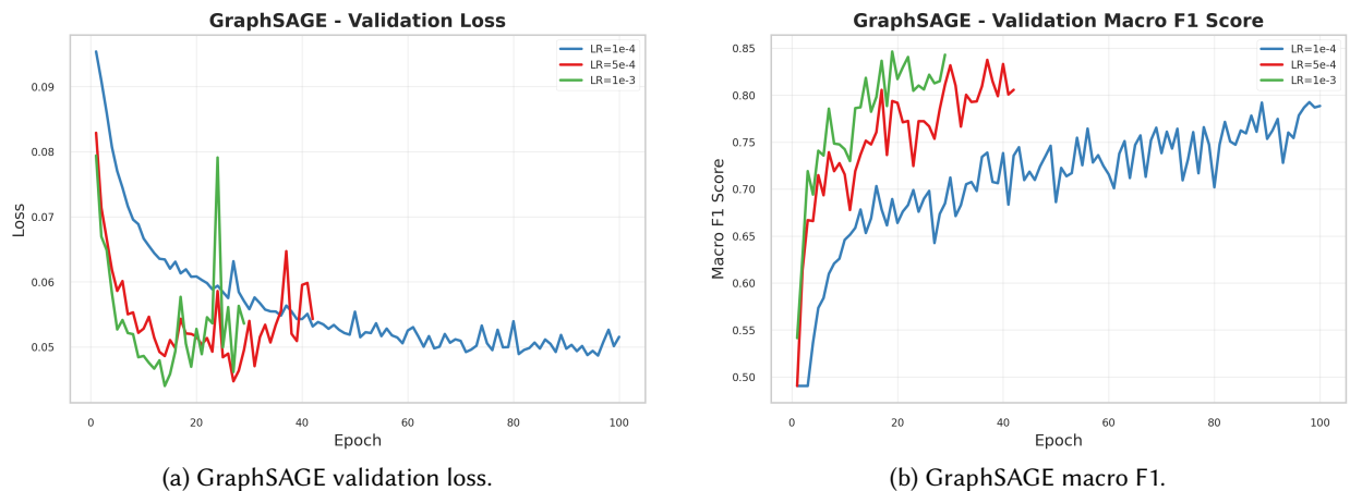
Fig. 9. Validation curves for GraphSAGE across learning rates.
