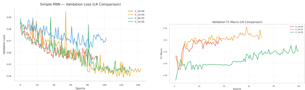
(a) Simple RNN validation loss.
