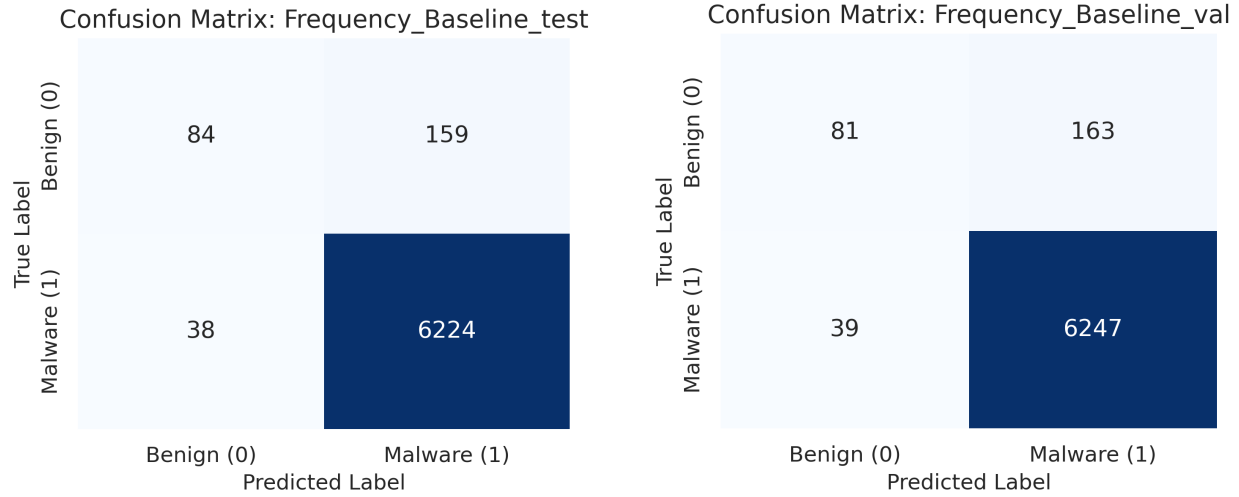
(a) Confusion matrix for the frequency-based baseline on the test set.
