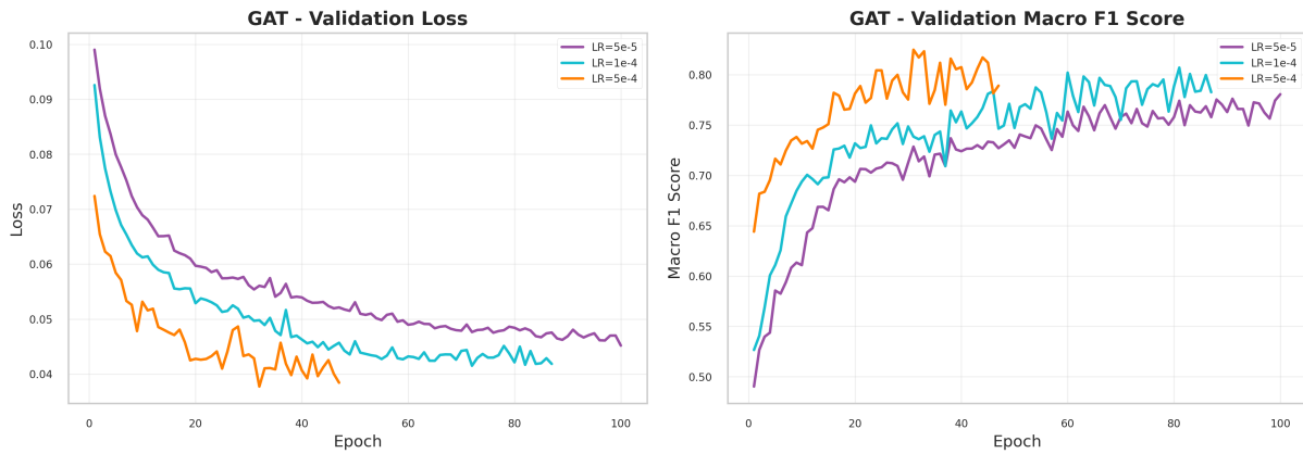
Fig. 8. Validation curves for GAT across learning rates.
