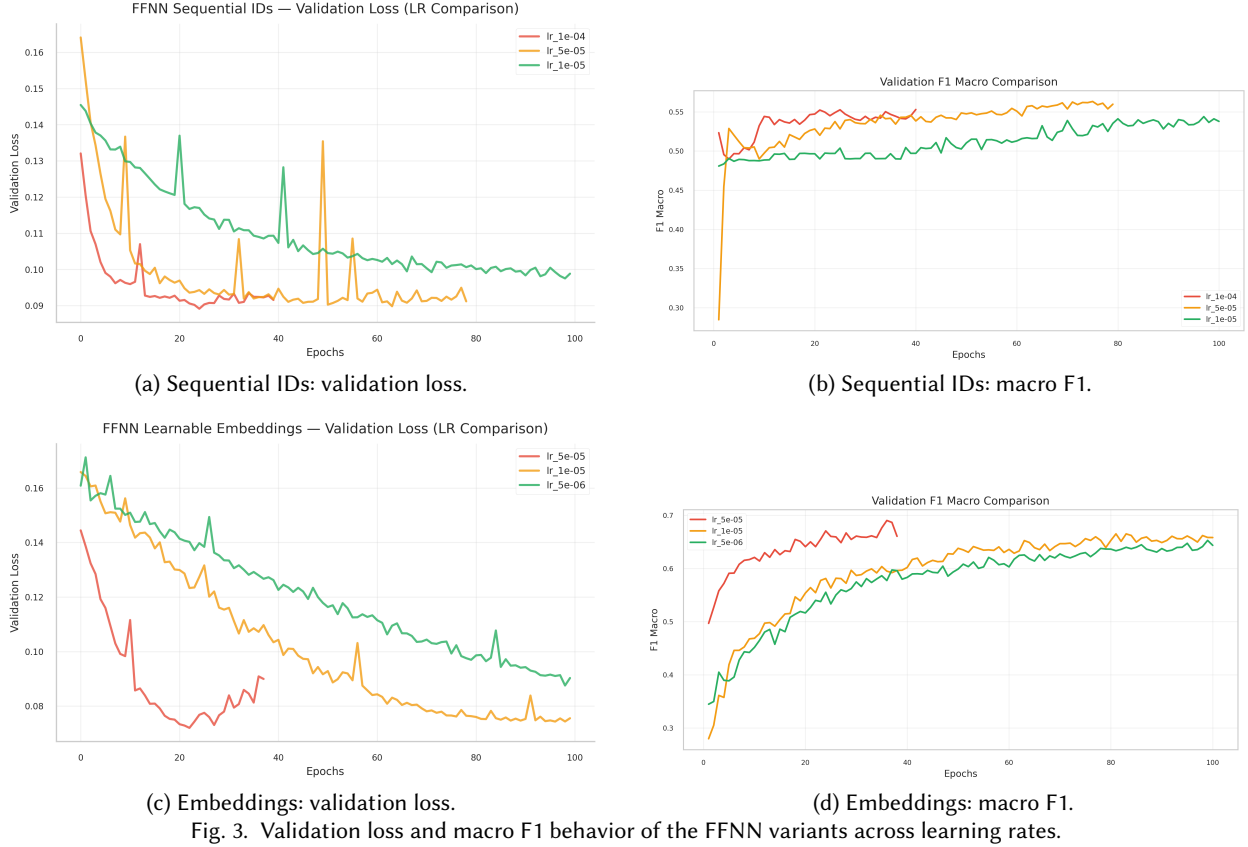
Fig. 3. Validation loss and macro F1 behavior of the FFNN variants across learning rates.
