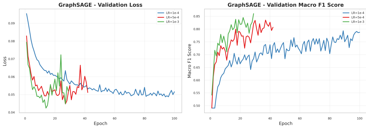
Fig. 7. Validation curves for GraphSAGE across learning rates.
