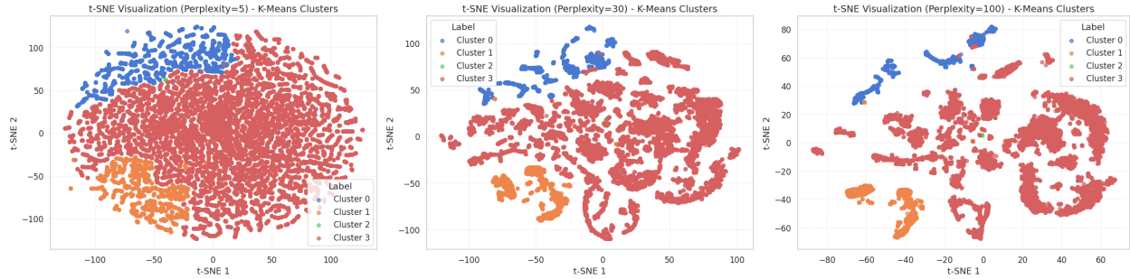
Fig. 8. t-SNE at three perplexity values. Perplexity = 5 over-fragments the data into micro-clusters; perplexity = 100 merges distinct attack islands; perplexity = 30 preserves both local separation and global structure.
