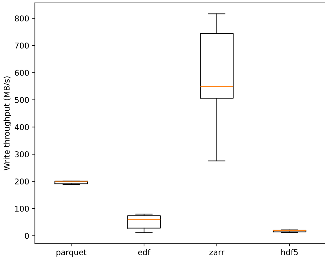
Experiment 2 - Write throughput by extension
