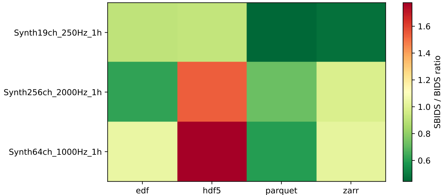
SBIDS vs BIDS speedup - Write latency (s)
