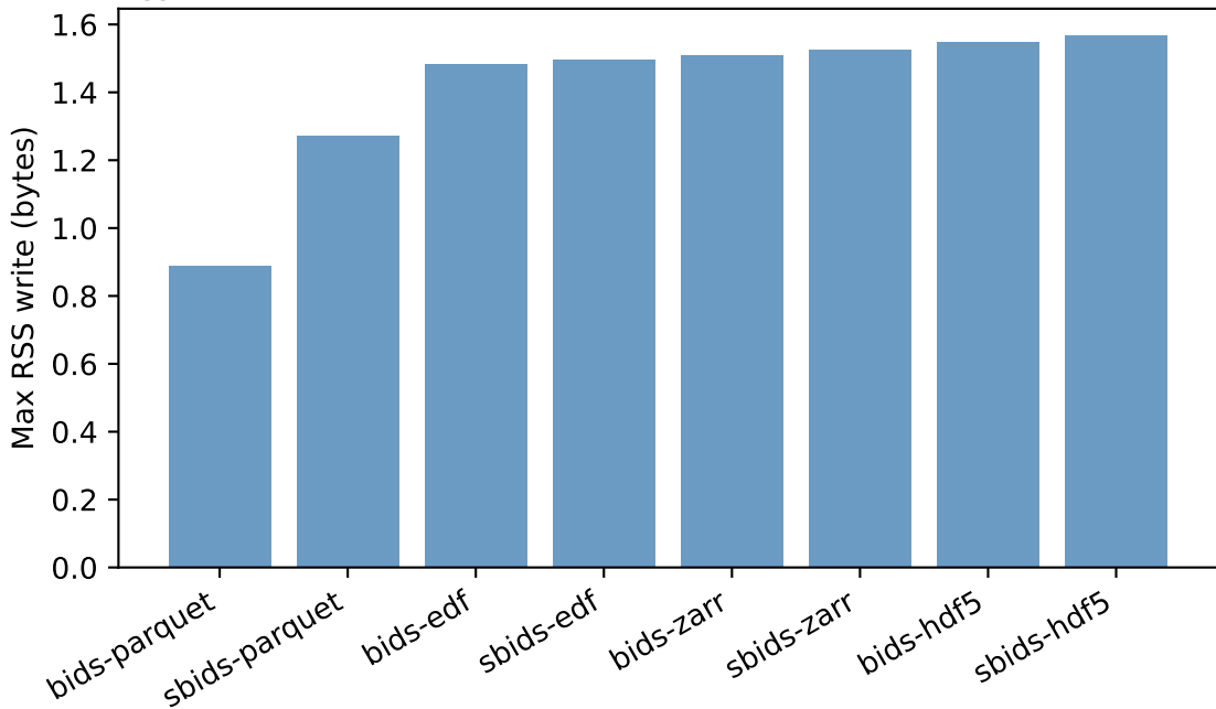
1e9 Synth Synth19ch_250Hz_1h - Max RSS write (bytes)
