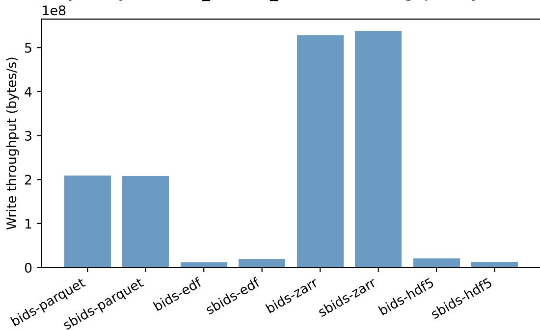
Synth Synth256ch_2000Hz_1h - Write throughput (bytes/s)
