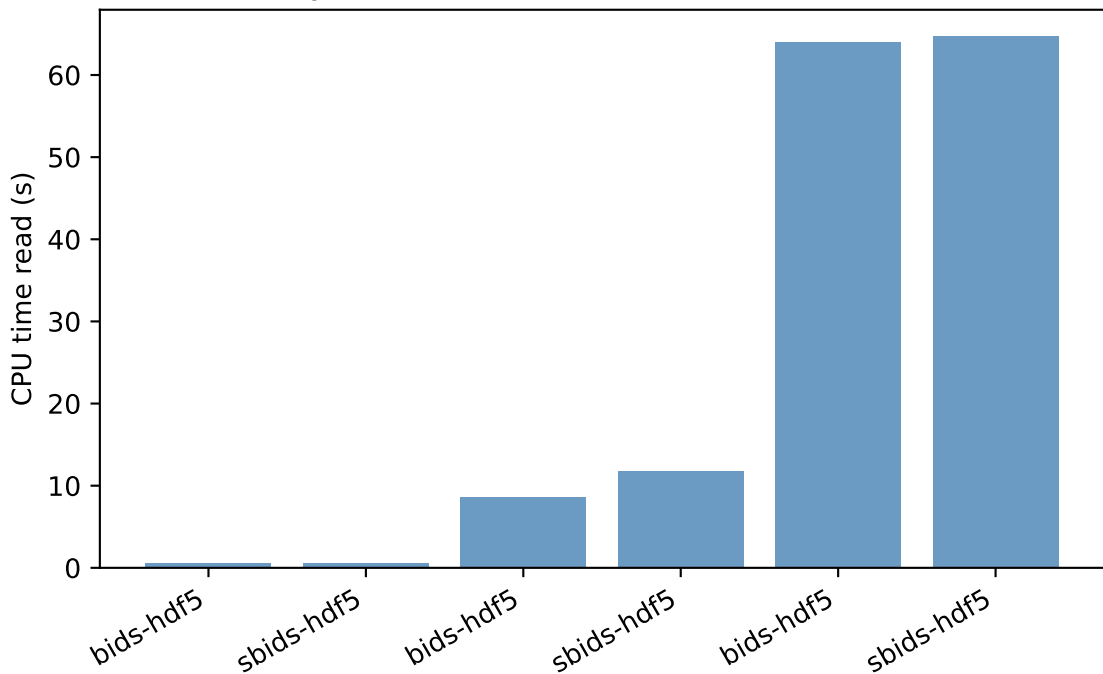
Synth format HDF5 - CPU time read (s)
