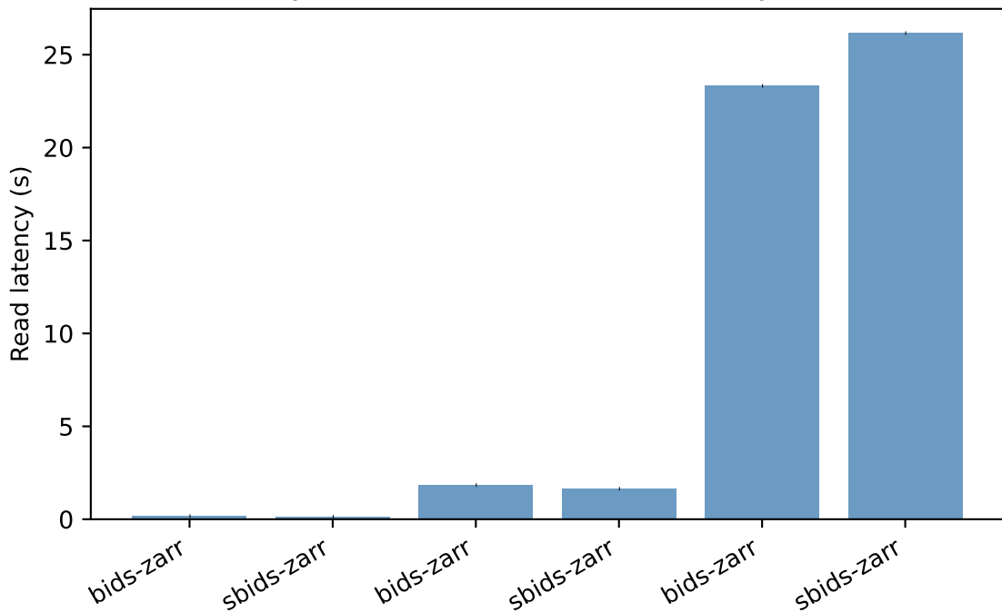
Synth format ZARR - Read latency (s)
