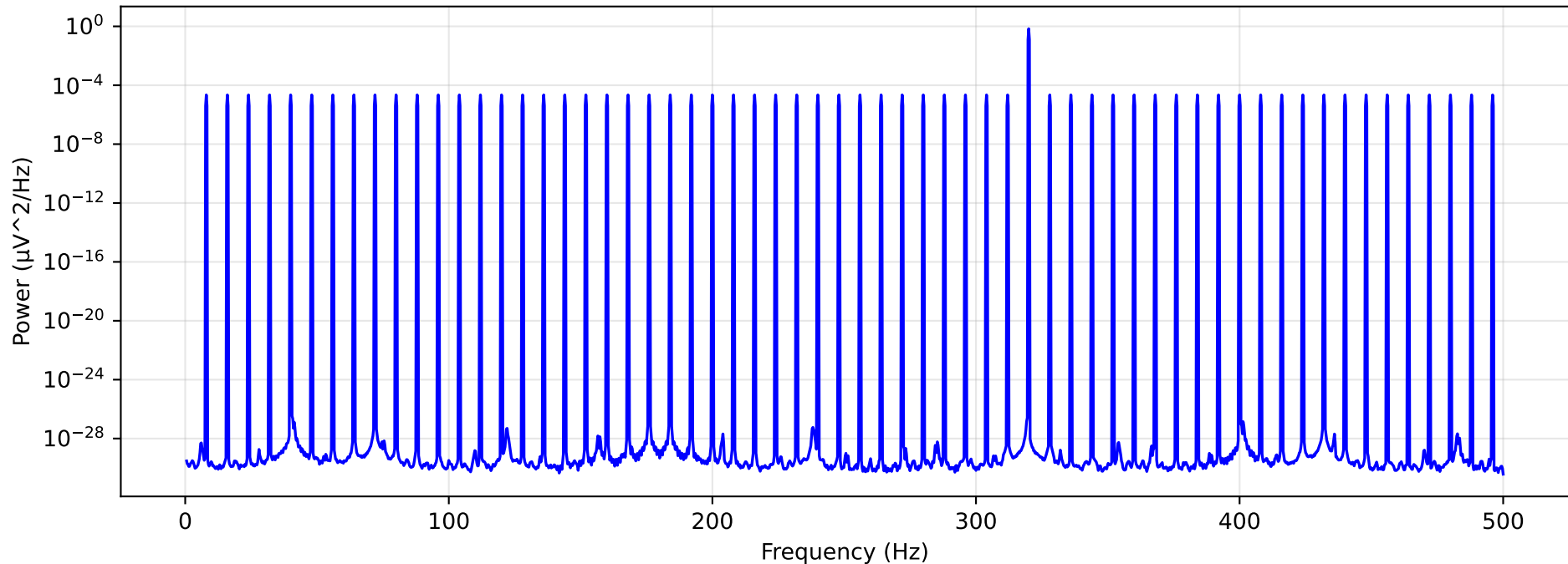
Sine PSD (mean across channels)
