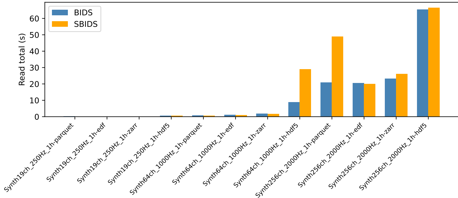
BIDS vs SBIDS - Read total (s)
