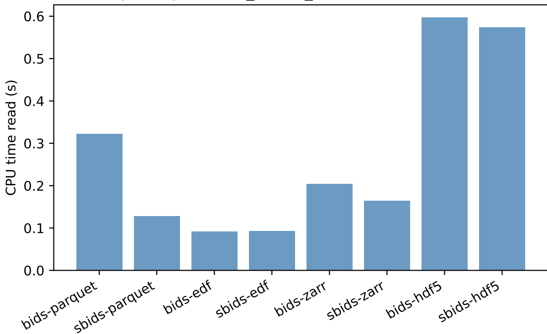
Synth Synth19ch_250Hz_1h - CPU time read (s)
