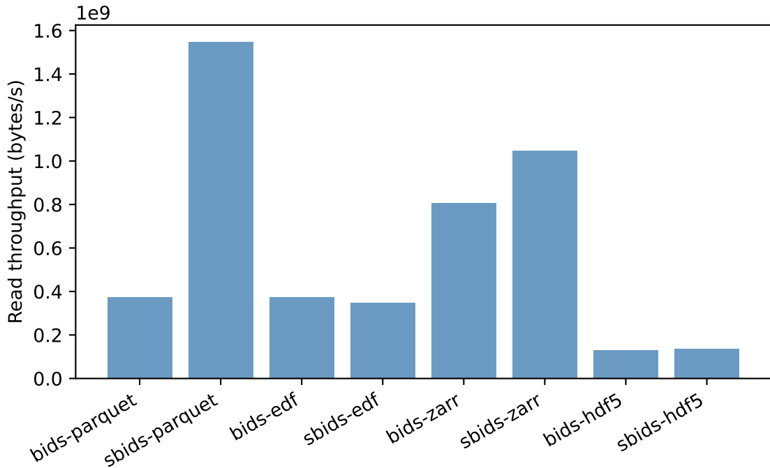
Synth Synth19ch_250Hz_1h - Read throughput (bytes/s)
