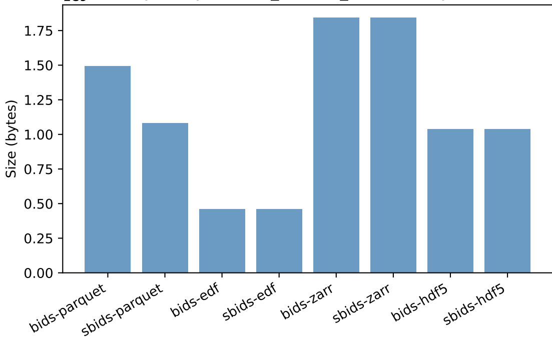
1e9 Synth Synth64ch_1000Hz_1h - Size (bytes)
