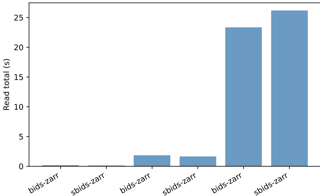
Synth format ZARR - Read total (s)
