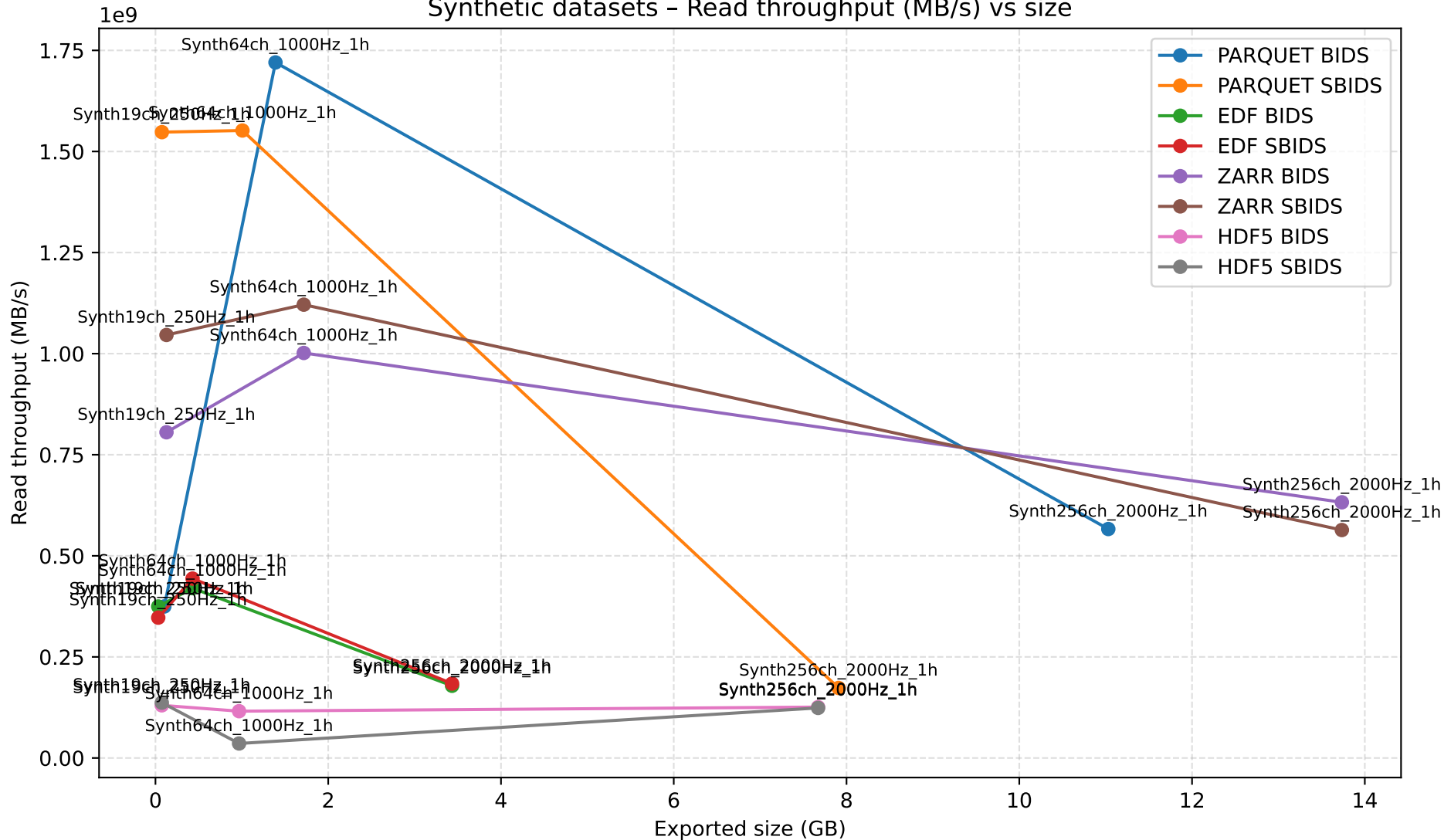
Synthetic datasets - Read throughput (MB/s) vs size
