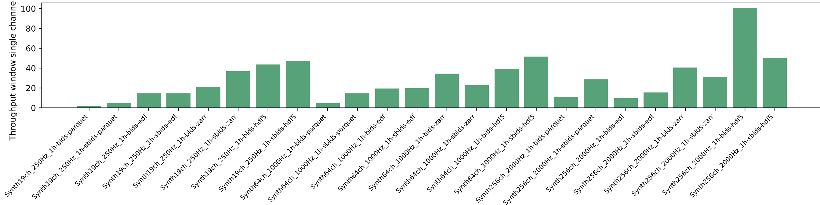
Streaming throughput - Throughput window single channel (MB/s)
