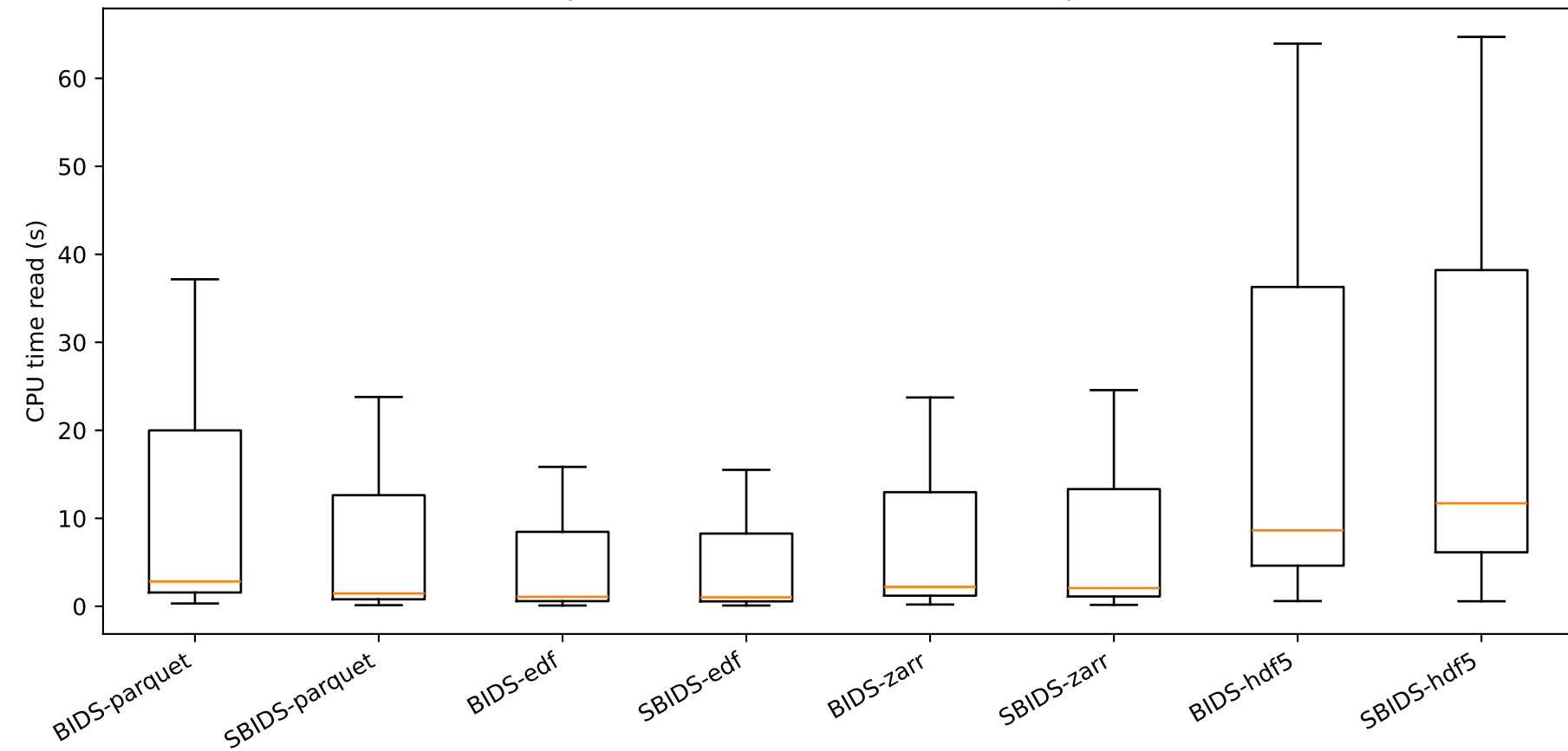
Experiment 2 - CPU time read (s) (boxplots)
