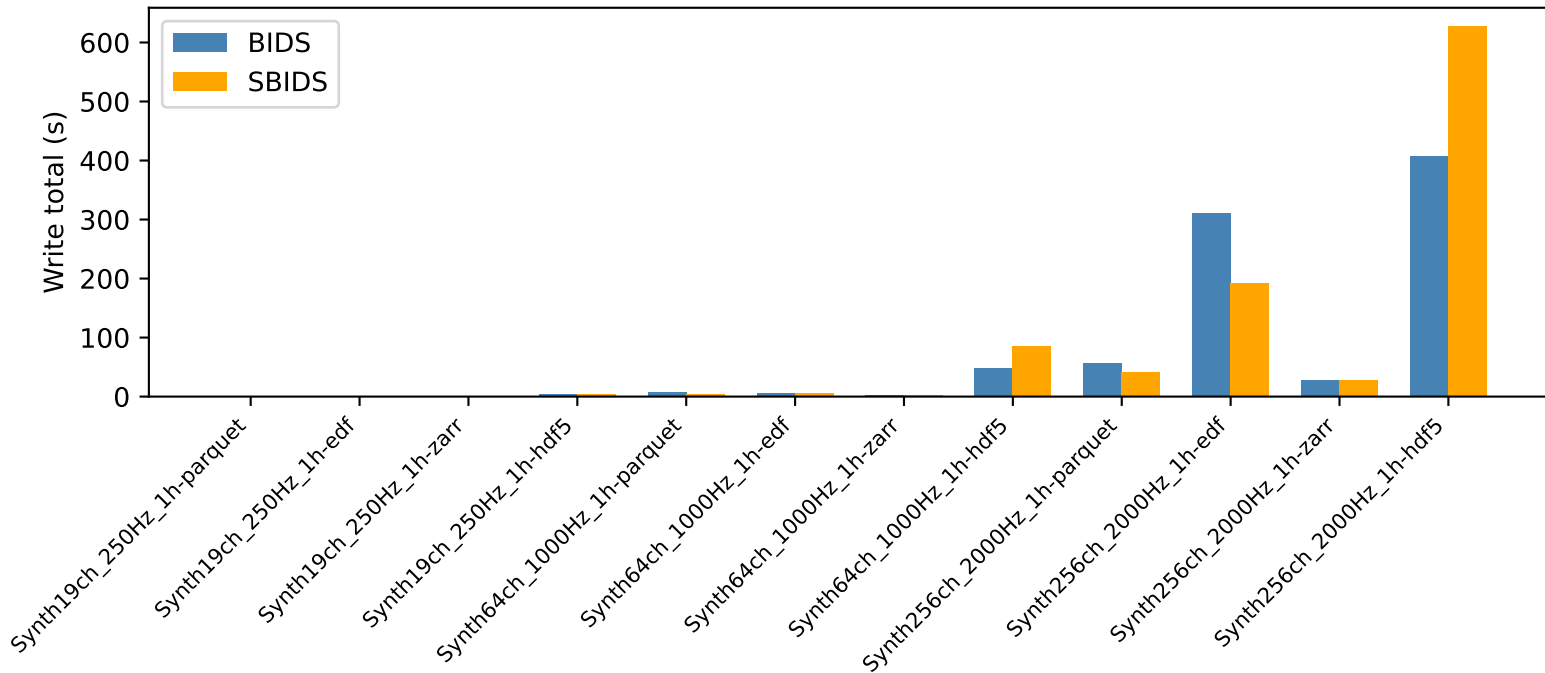
BIDS vs SBIDS - Write total (s)
