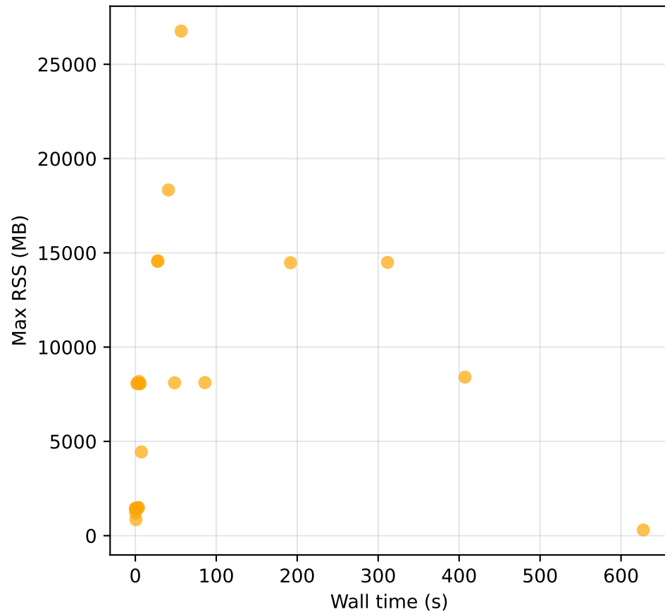
Write: RSS vs wall
