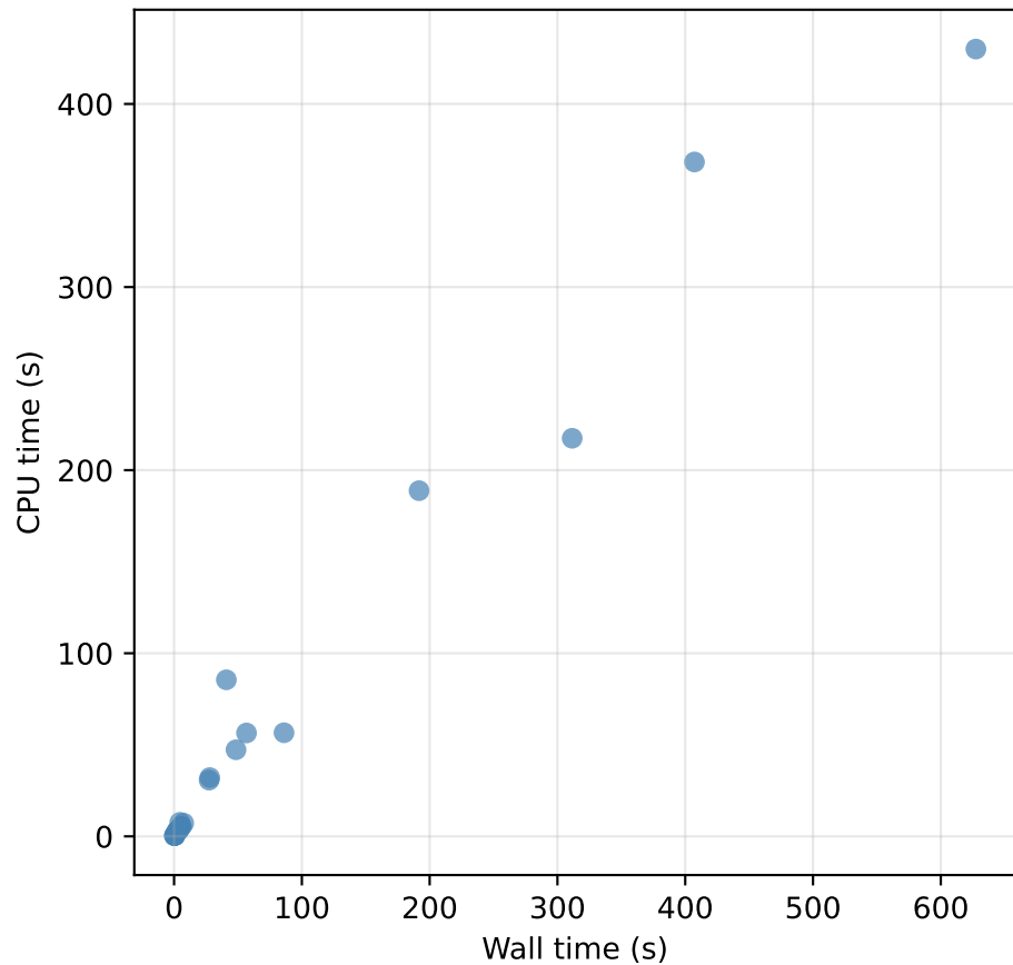
Write: CPU vs wall
