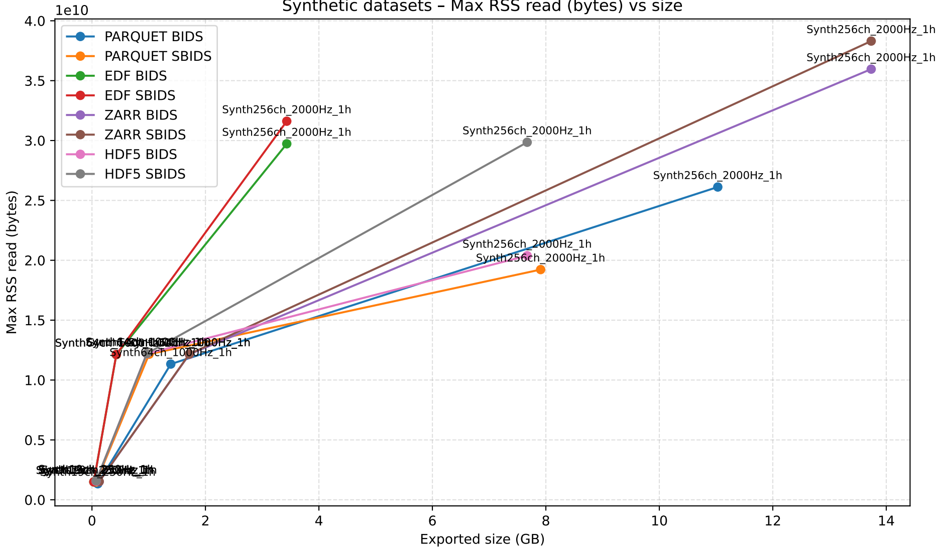
Synthetic datasets - Max RSS read (bytes) vs size
