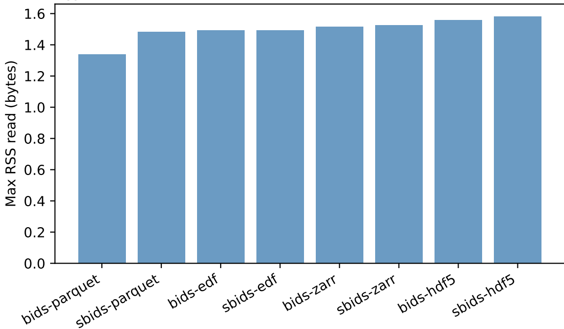
1e9 Synth Synth19ch_250Hz_1h - Max RSS read (bytes)
