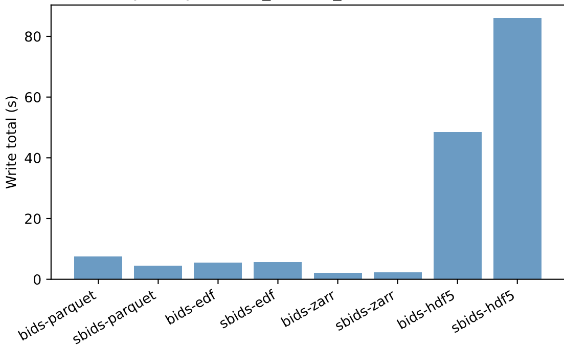
Synth Synth64ch_1000Hz_1h - Write total (s)
